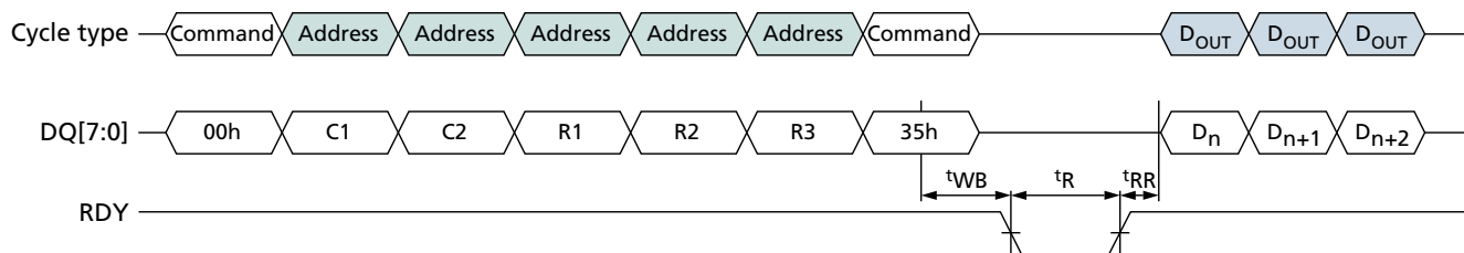
Figure 56: COPYBACK READ (00h-35h) with CHANGE READ COLUMN (05h-E0h) Operation
