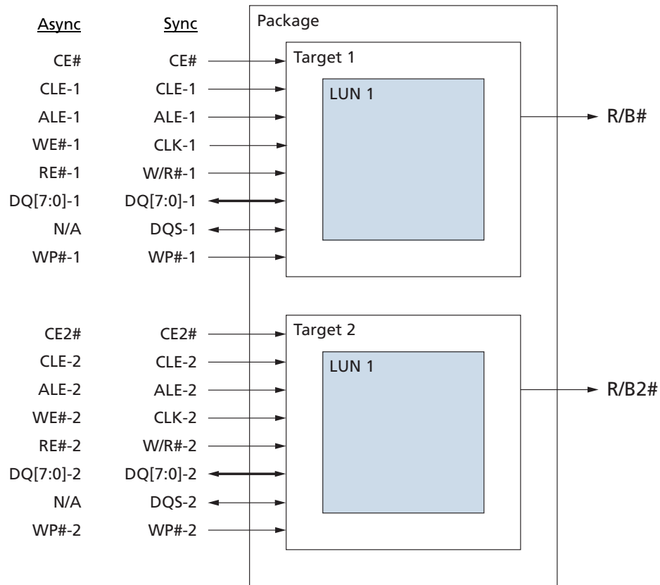
Figure 7: Device Organization for Two-Die Package (BGA)
