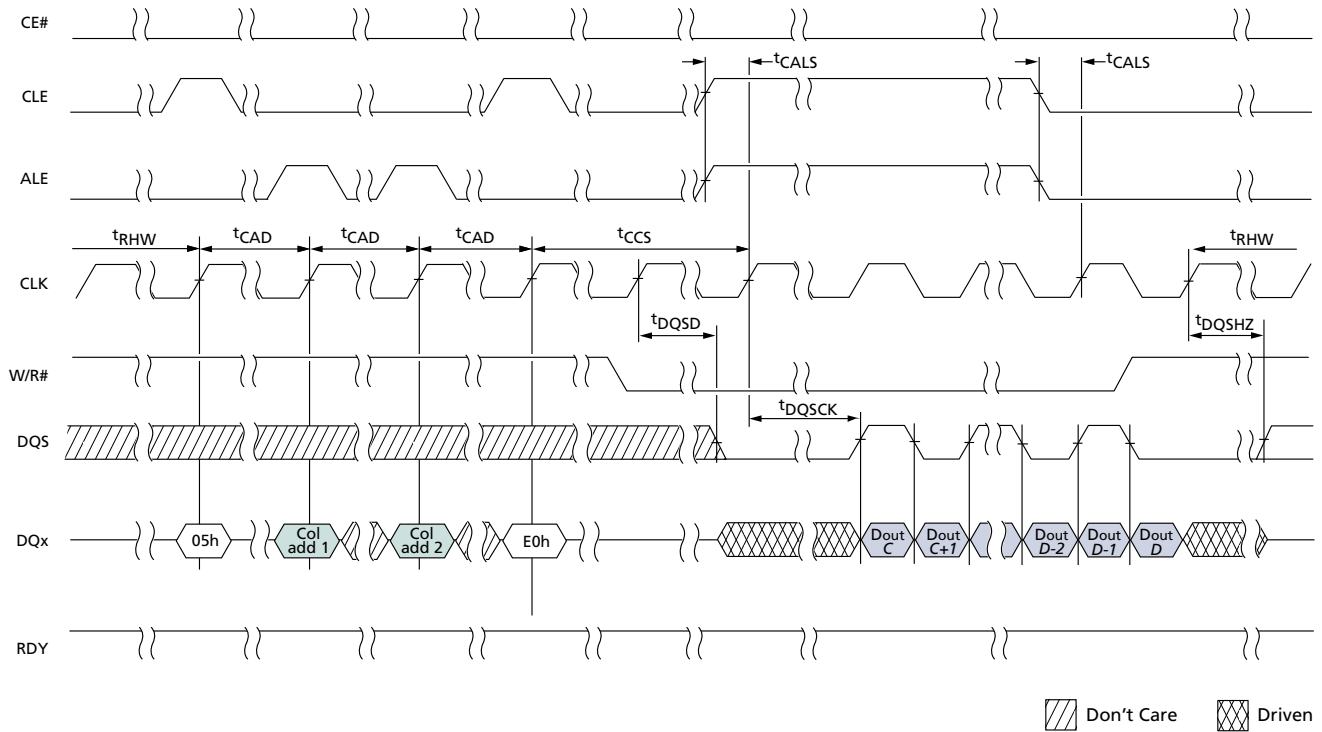
Figure 91: CHANGE READ COLUMN
