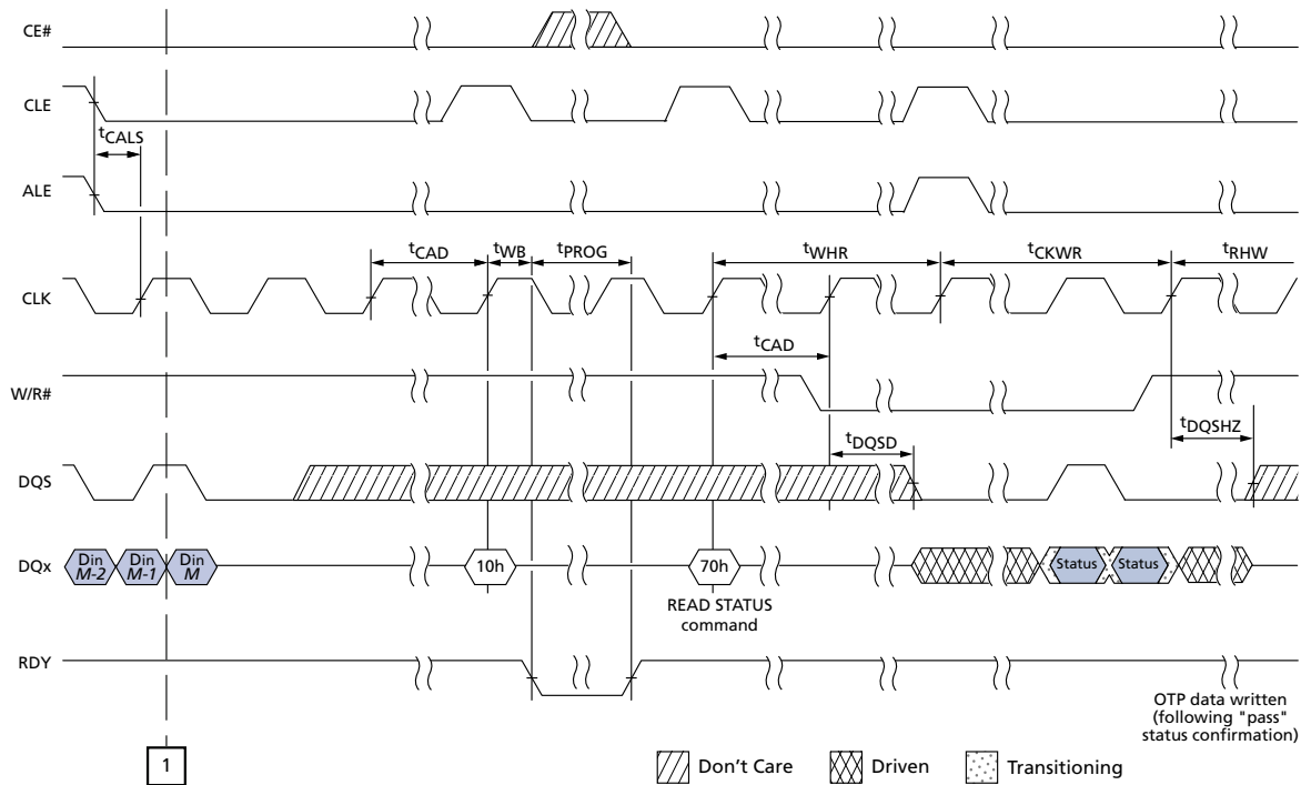
Figure 108: PROGRAM OTP PAGE (2 of 2)
