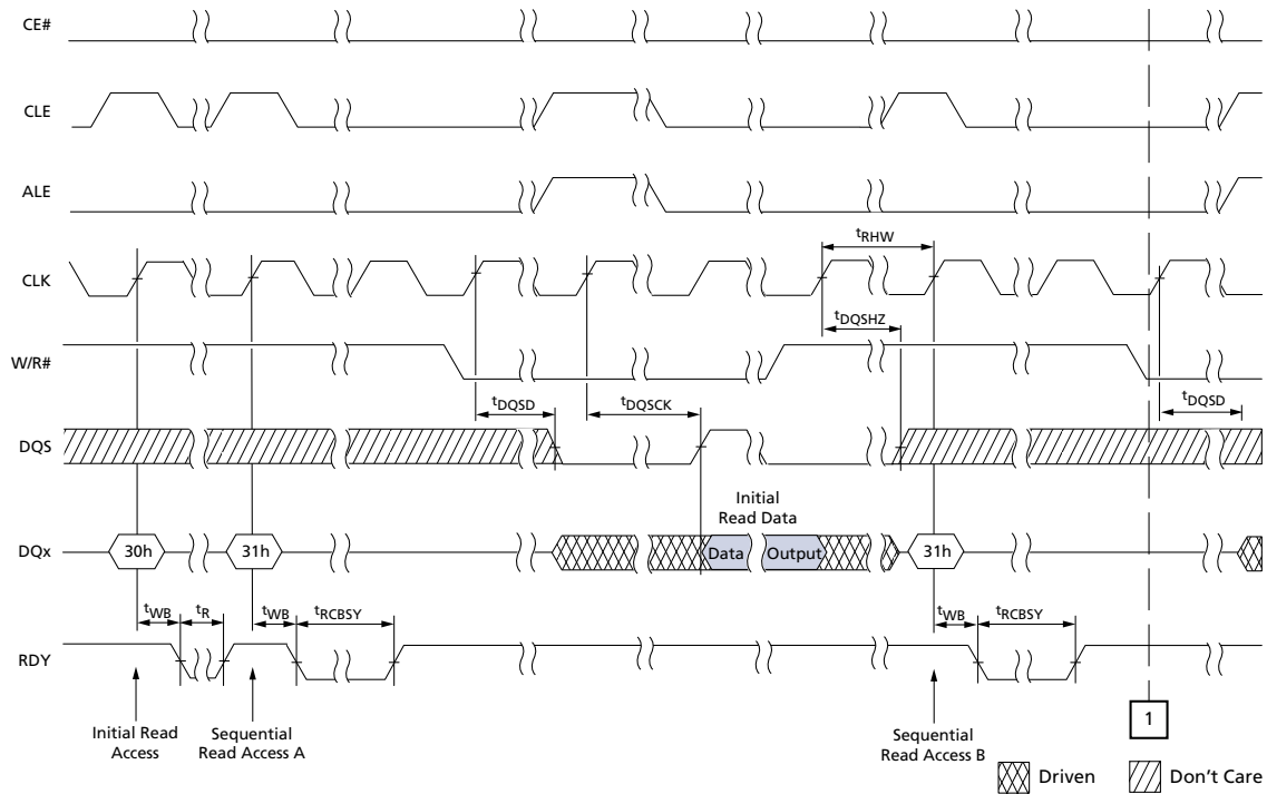
Figure 92: READ PAGE CACHE SEQUENTIAL (1 of 2)
