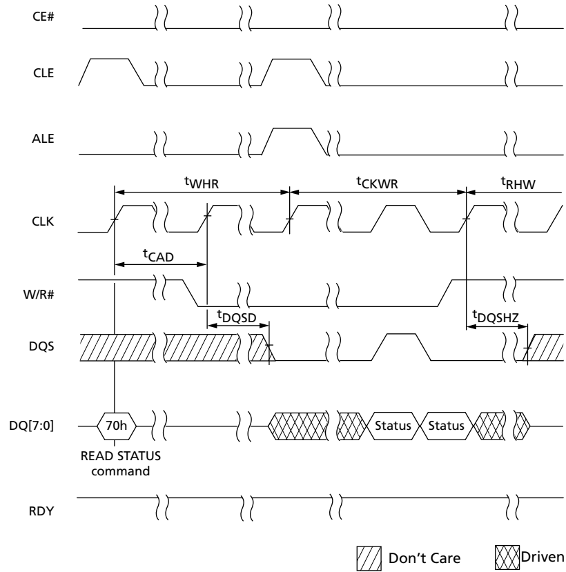
Figure 87: READ STATUS Cycle
