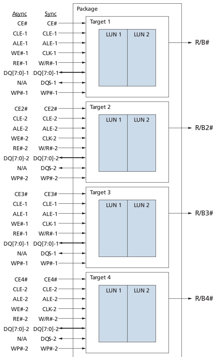
Figure 10: Device Organization for Eight-Die Package (BGA)
