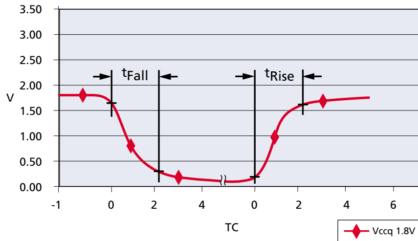
Figure 19: t_{\text{Fall}} and t_{\text{Rise}} ( V_{\text{CCQ}} = 1.7\text{-}1.95\text{V} )
