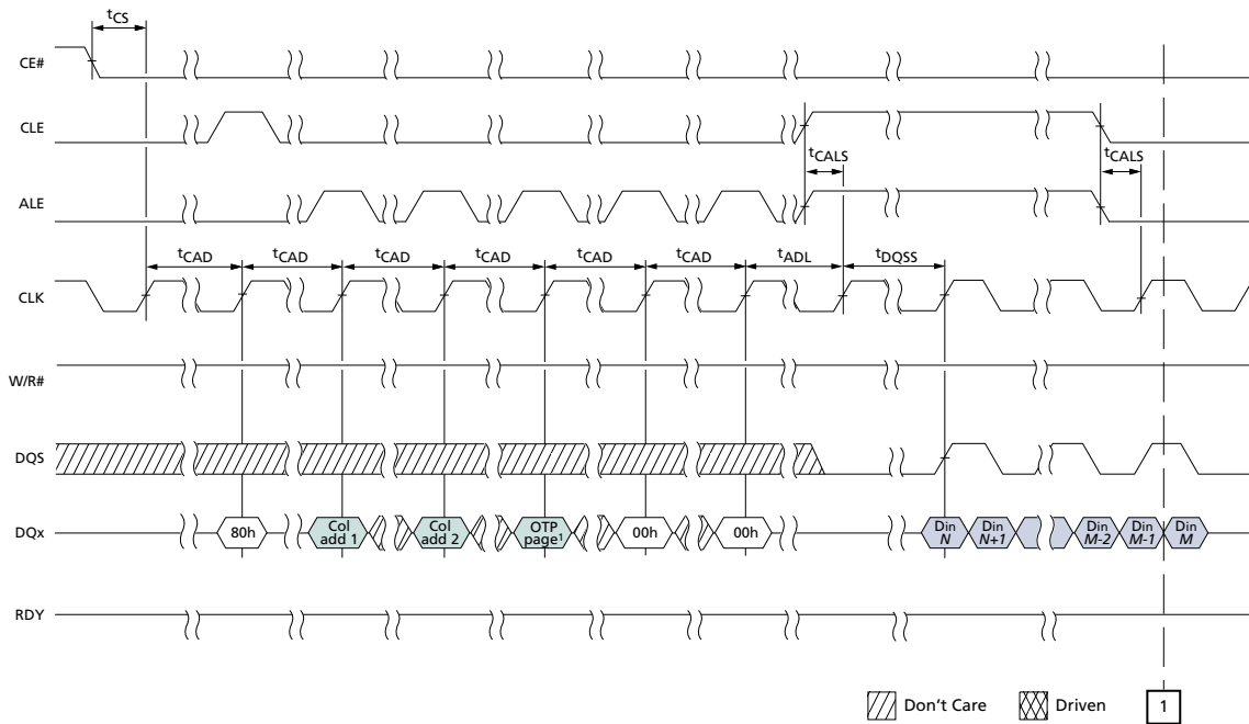
Figure 108: PROGRAM OTP PAGE (2 of 2)
