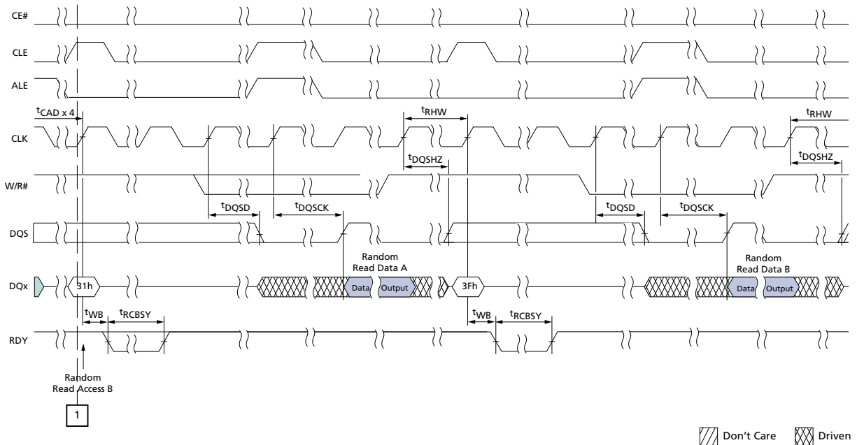
Figure 95: READ PAGE CACHE RANDOM (2 of 2)
