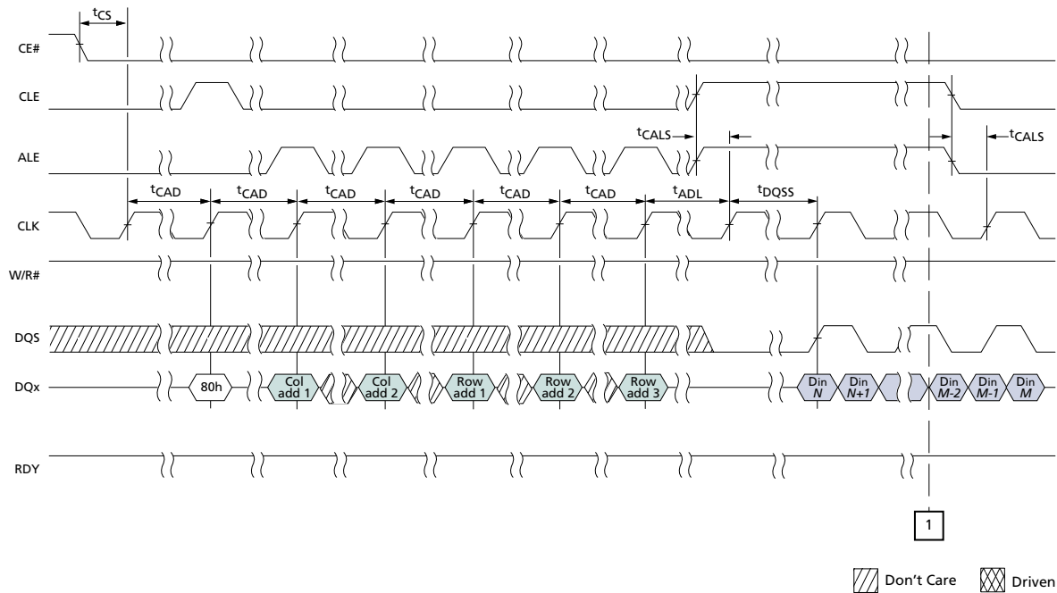
Figure 99: PROGRAM PAGE Operation (2 of 2)
