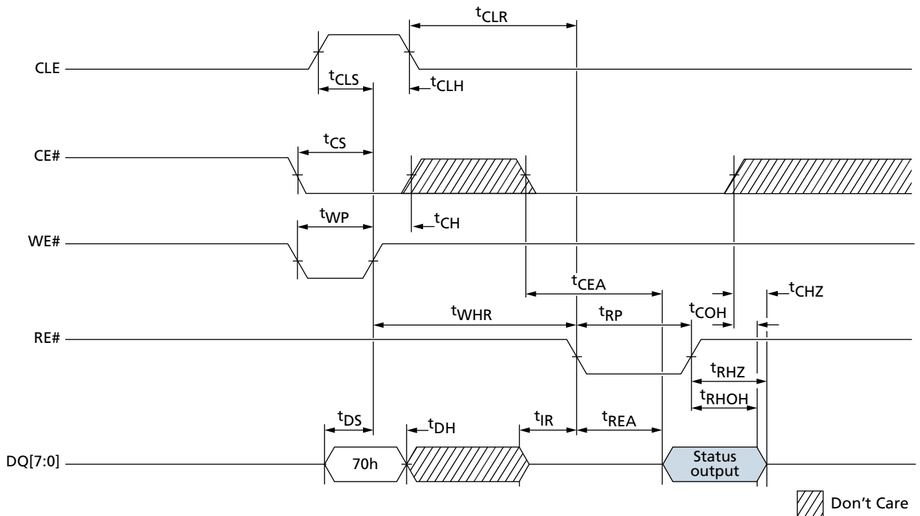
Figure 67: READ STATUS Cycle
