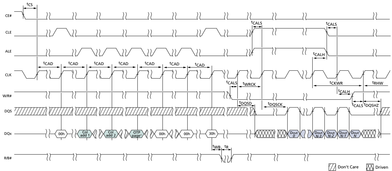
Figure 106: READ OTP PAGE
