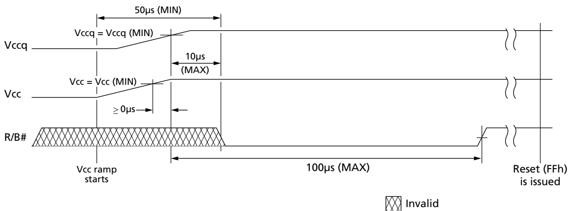
Figure 28: R/B# Power-On Behavior
