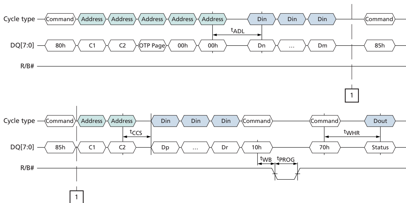
Figure 61: PROGRAM OTP PAGE (80h-10h) with CHANGE WRITE COLUMN (85h) Operation
