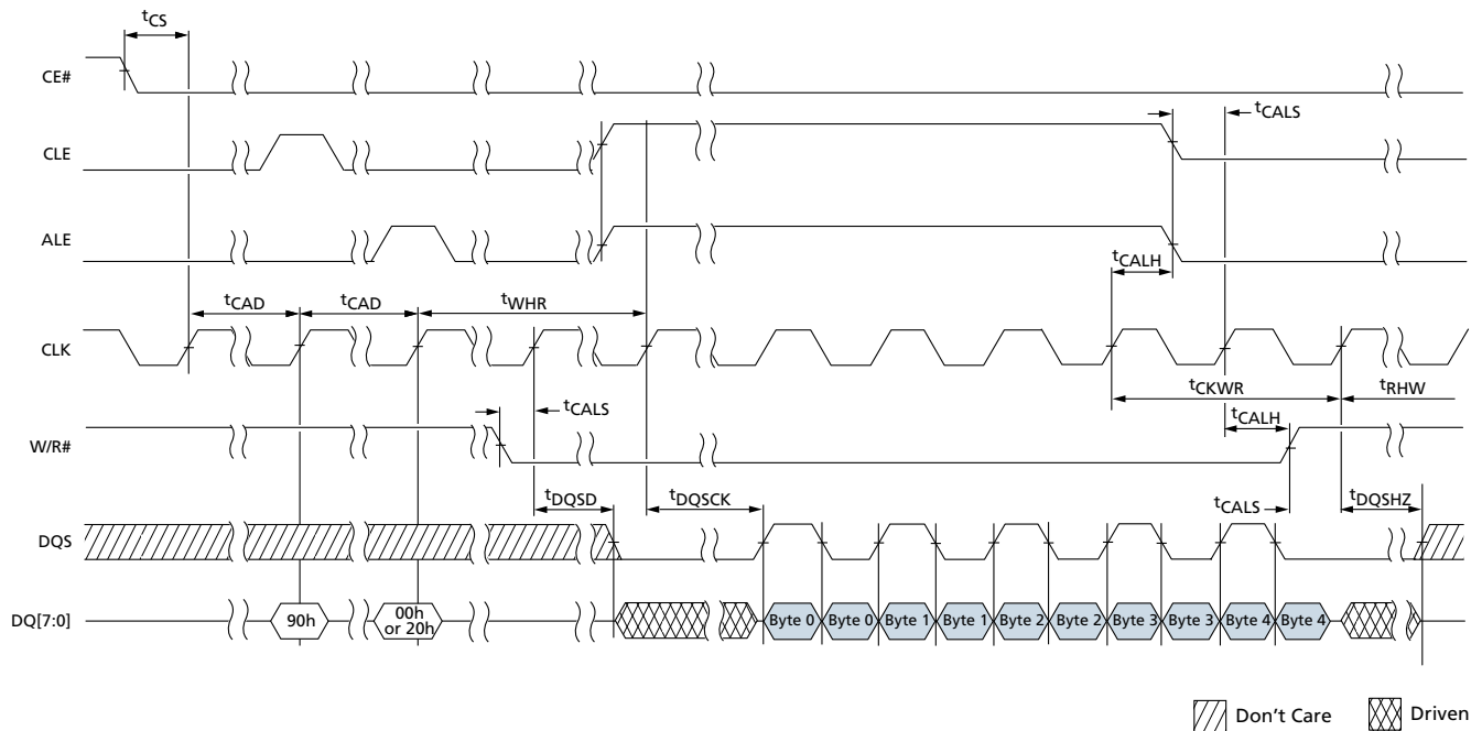
Figure 84: READ ID Operation
