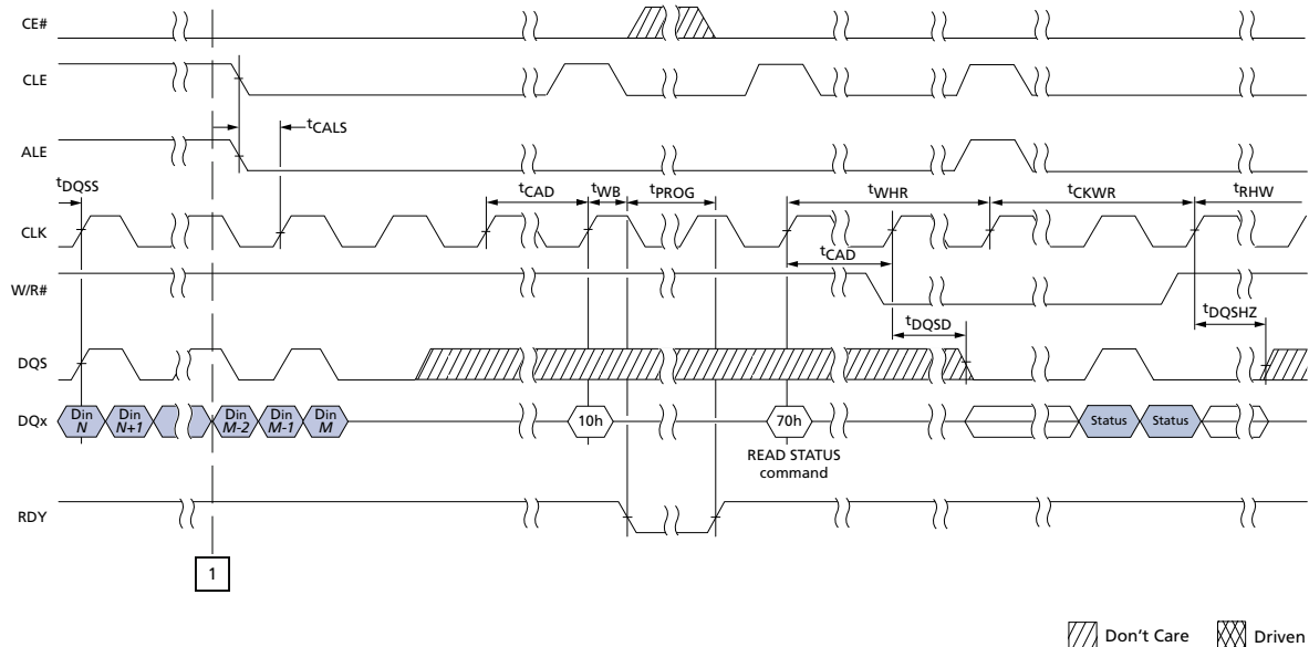
Figure 99: PROGRAM PAGE Operation (2 of 2)
