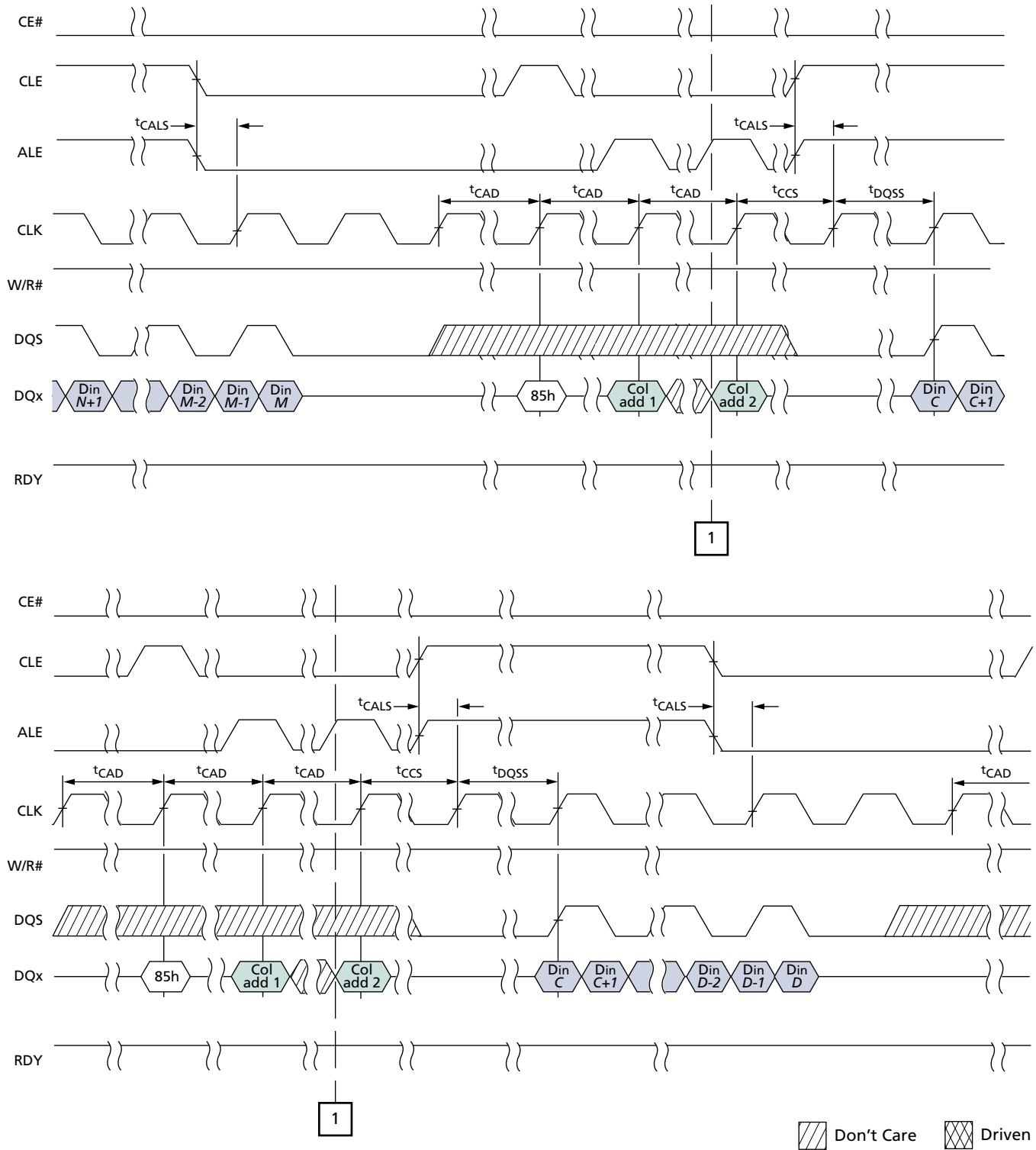
Figure 100: CHANGE WRITE COLUMN
