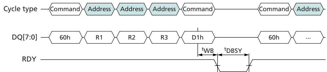
Figure 54: ERASE BLOCK MULTI-PLANE (60h-D1h) Operation
