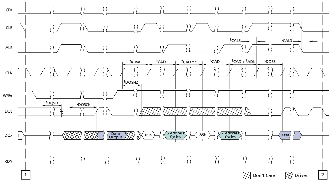
Figure 105: COPYBACK (3 of 3)
