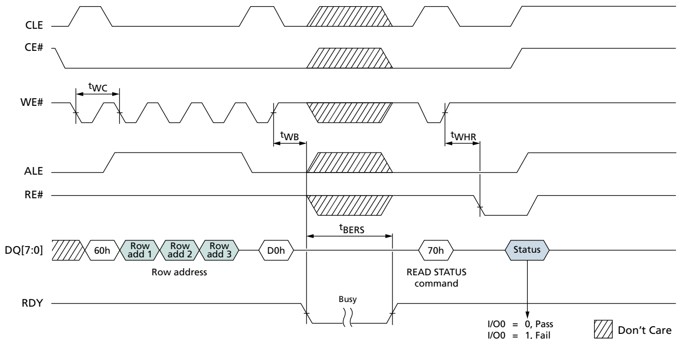
Figure 82: ERASE BLOCK Operation
