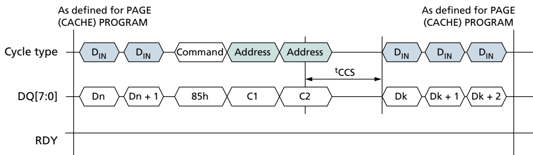
Figure 42: CHANGE WRITE COLUMN (85h) Operation
