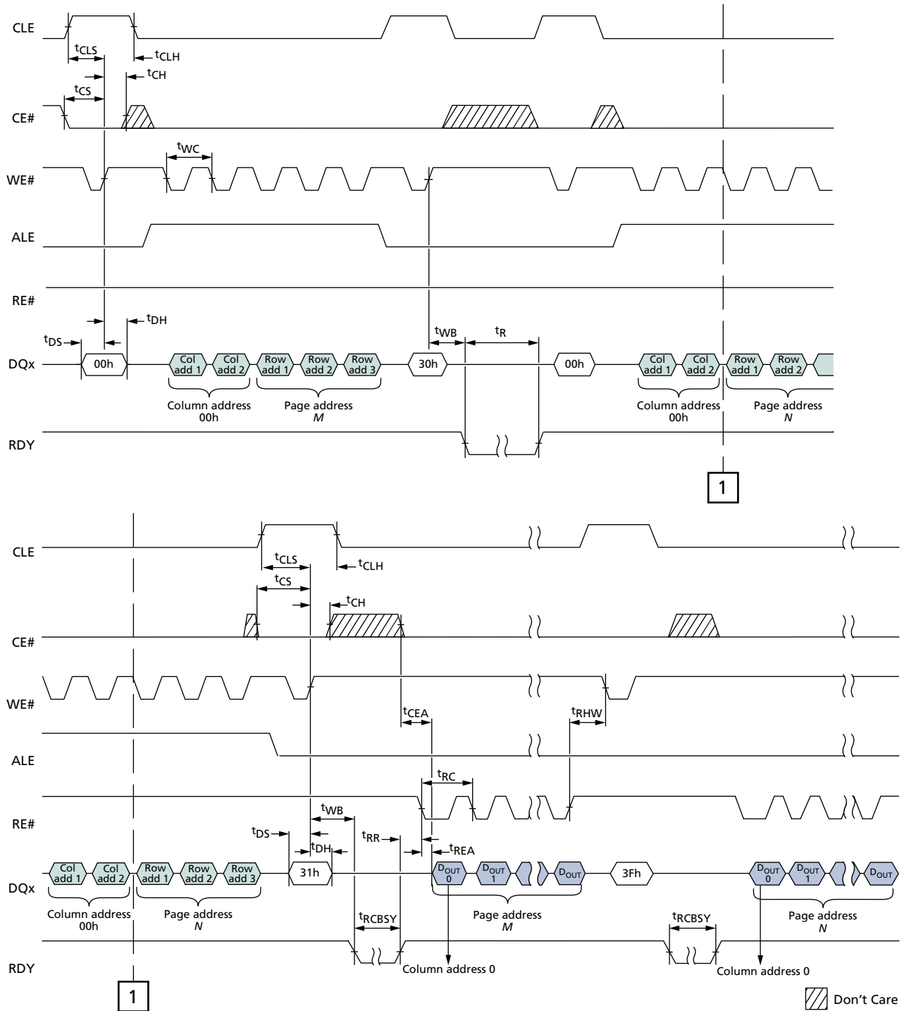
Figure 74: READ PAGE CACHE RANDOM
