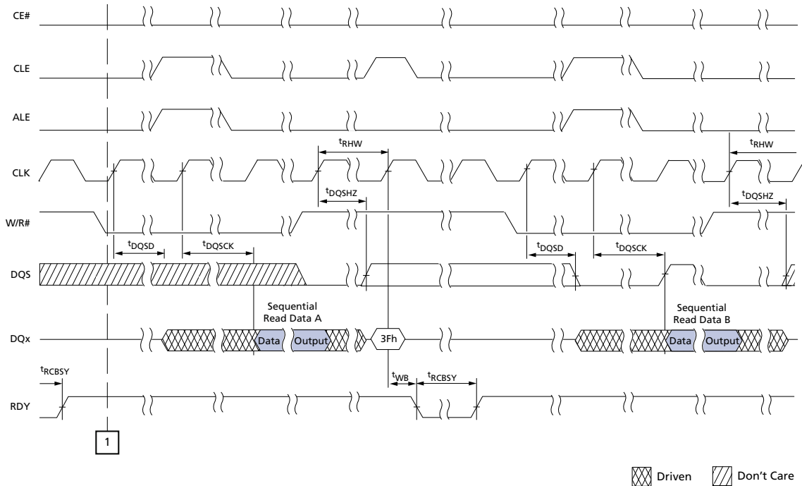
Figure 93: READ PAGE CACHE SEQUENTIAL (2 of 2)
