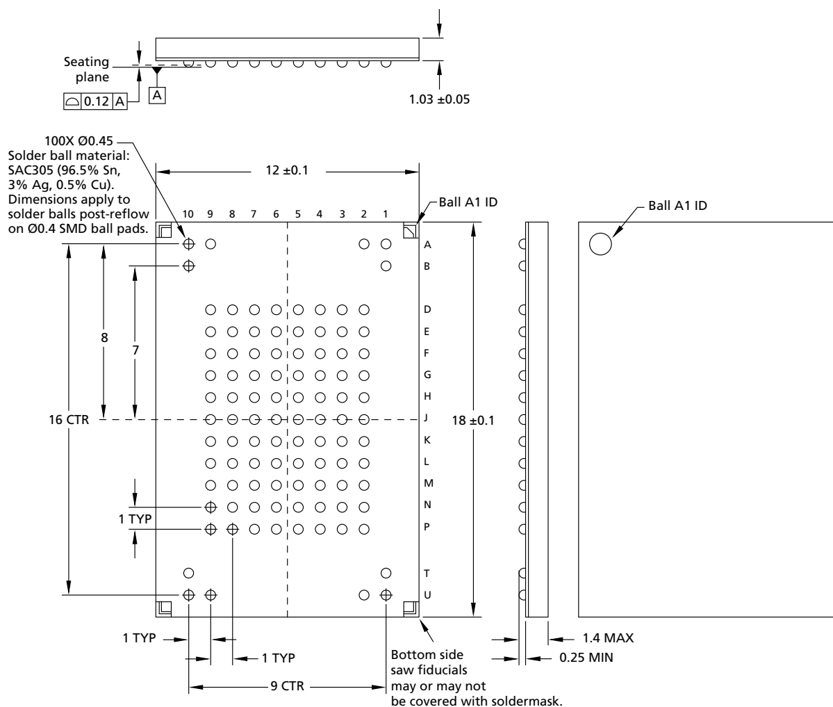
Figure 5: 100-Ball LBGA – 12mm x 18mm (Package Code: H3)
