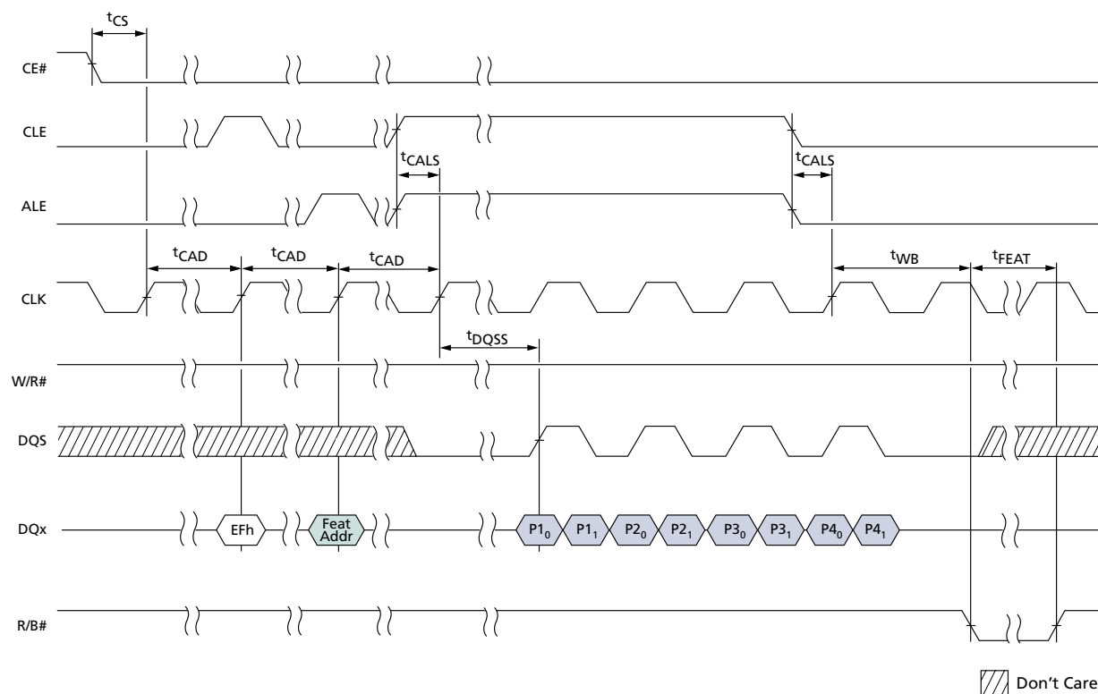
Figure 83: SET FEATURES Operation
