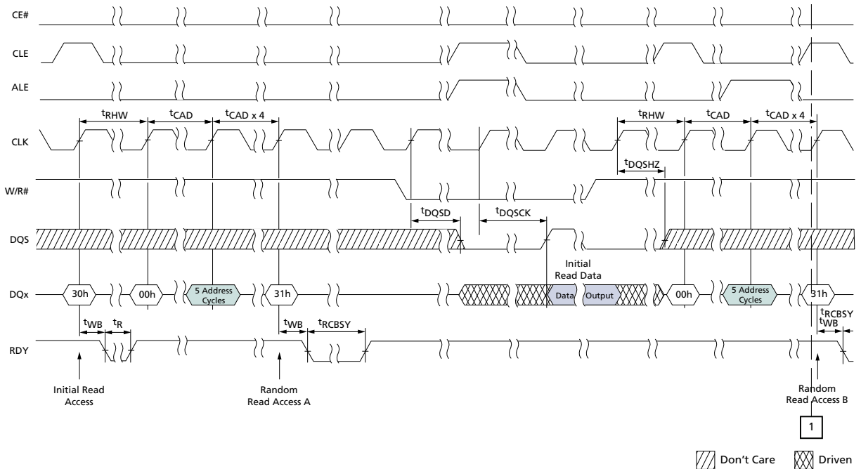
Figure 95: READ PAGE CACHE RANDOM (2 of 2)
