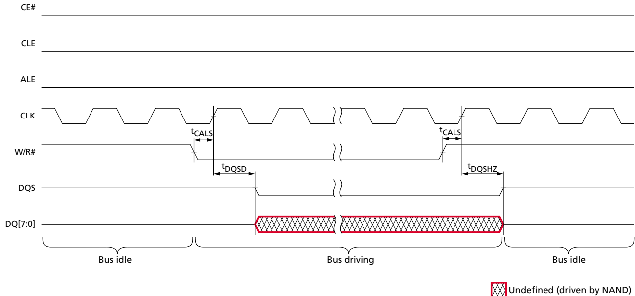
Figure 23: Synchronous Bus Idle/Driving Behavior
