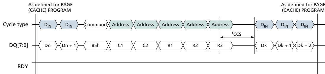
Figure 43: CHANGE ROW ADDRESS (85h) Operation
