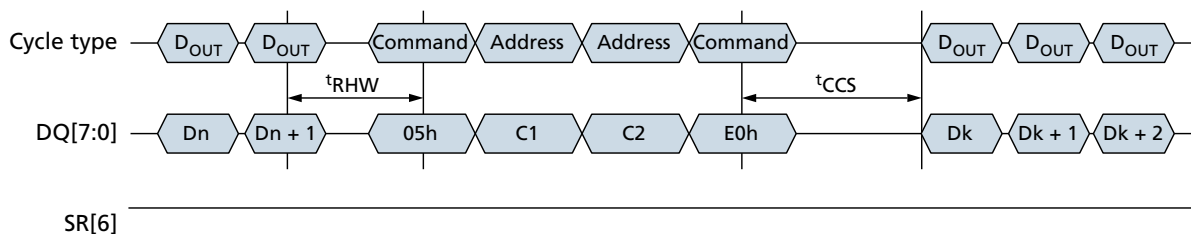
Figure 40: CHANGE READ COLUMN (05h-E0h) Operation
