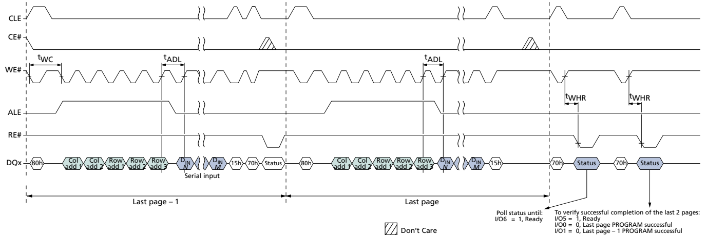
Figure 80: PROGRAM PAGE CACHE Ending on 15h
