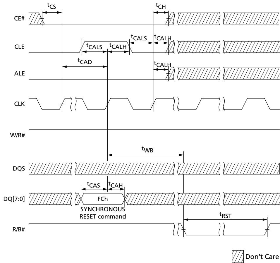
Figure 86: RESET (FCh) Operation
