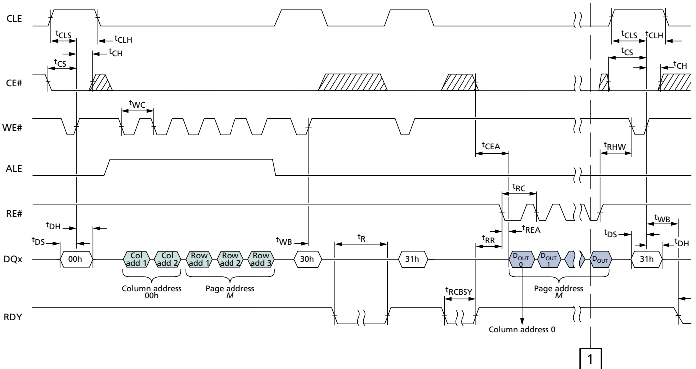
Figure 73: READ PAGE CACHE SEQUENTIAL
