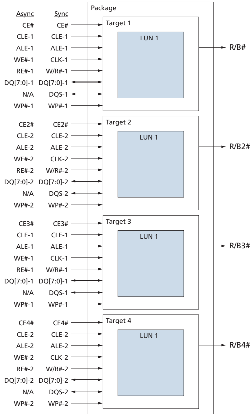
Figure 9: Device Organization for Four-Die Package with CE#, CE2#, CE3#, and CE4# (BGA)
