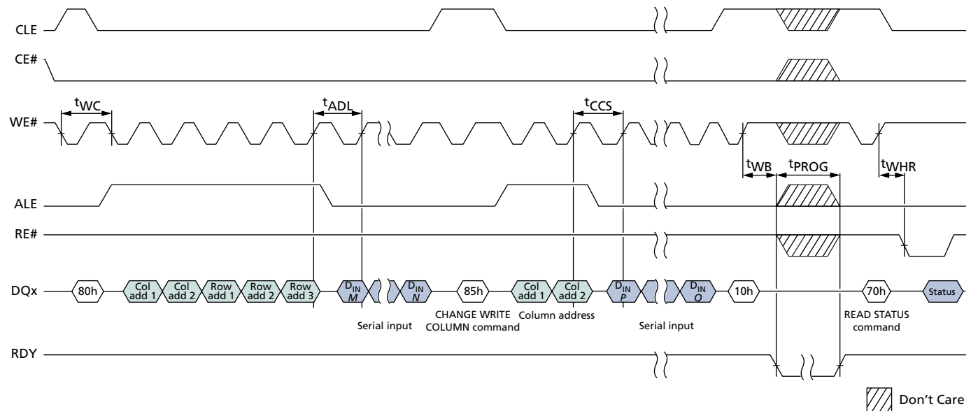
Figure 78: PROGRAM PAGE Operation with CHANGE WRITE COLUMN
