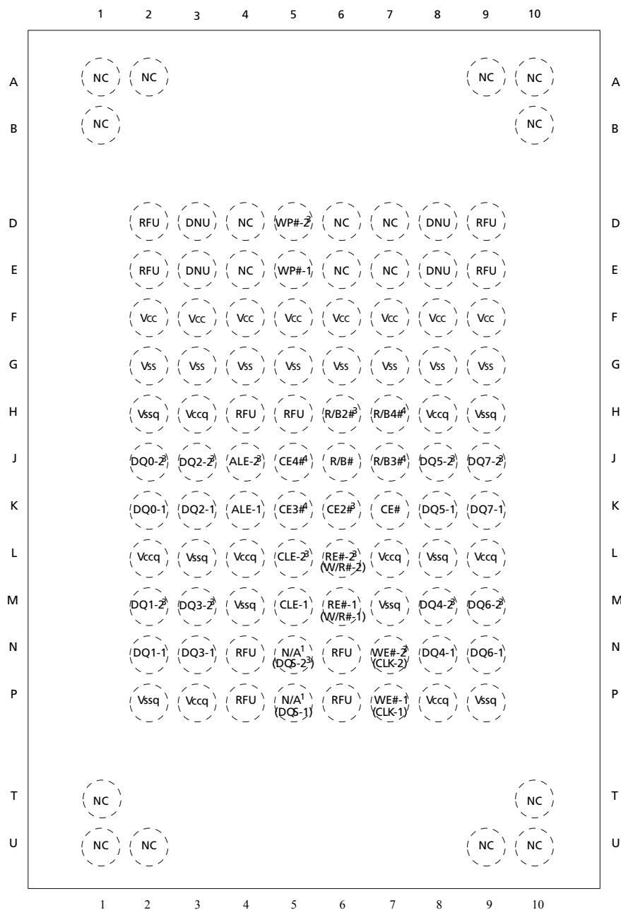
Figure 2: 100-Ball BGA (Ball-Down, Top View)
