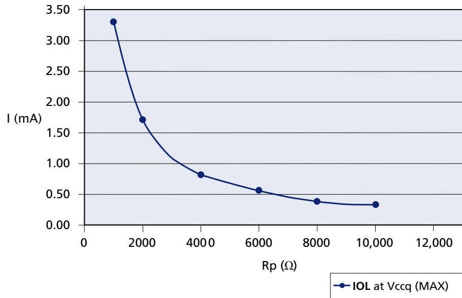
Figure 21: IOL vs Rp ( V_{CCQ} = 1.7\text{-}1.95\text{V} )
