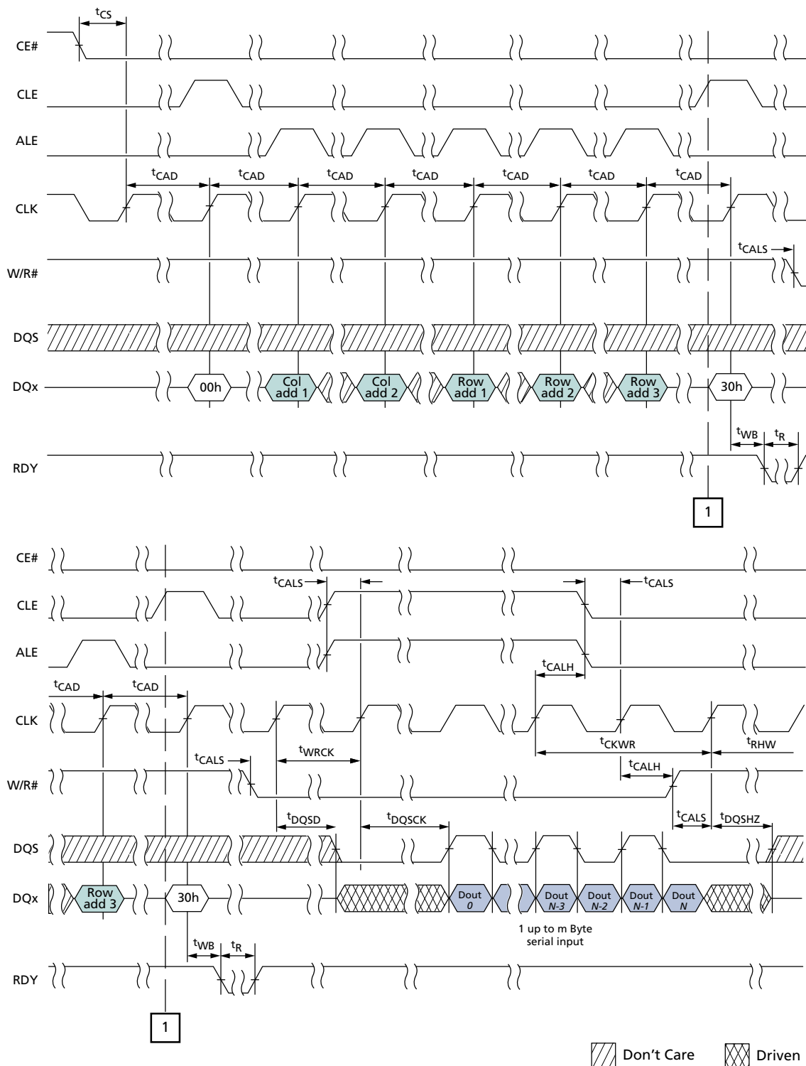
Figure 90: READ PAGE Operation
