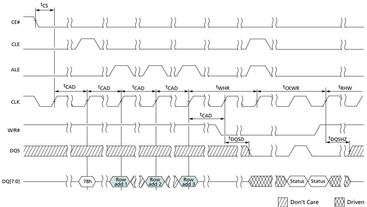
Figure 88: READ STATUS ENHANCED Operation
