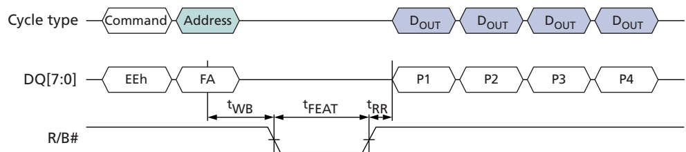
Figure 35: GET FEATURES (EEh) Operation
