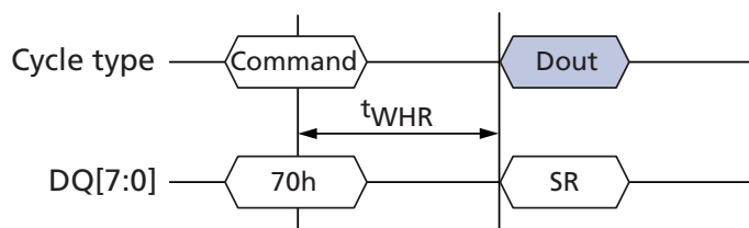
Figure 38: READ STATUS (70h) Operation
