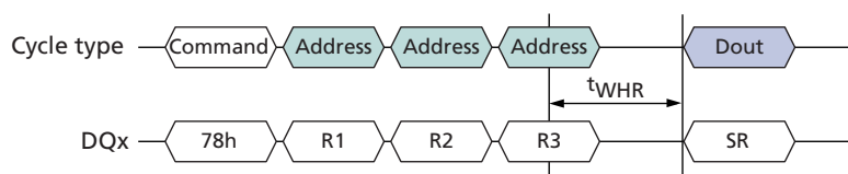
Figure 39: READ STATUS ENHANCED (78h) Operation
