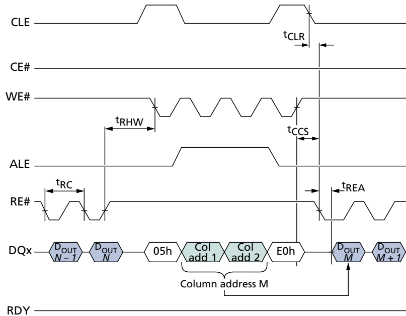
Figure 72: CHANGE READ COLUMN
