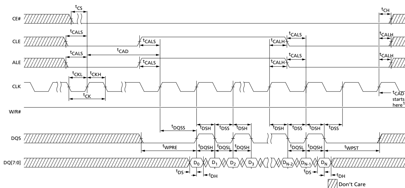
Figure 26: Synchronous DDR Data Input Cycles
