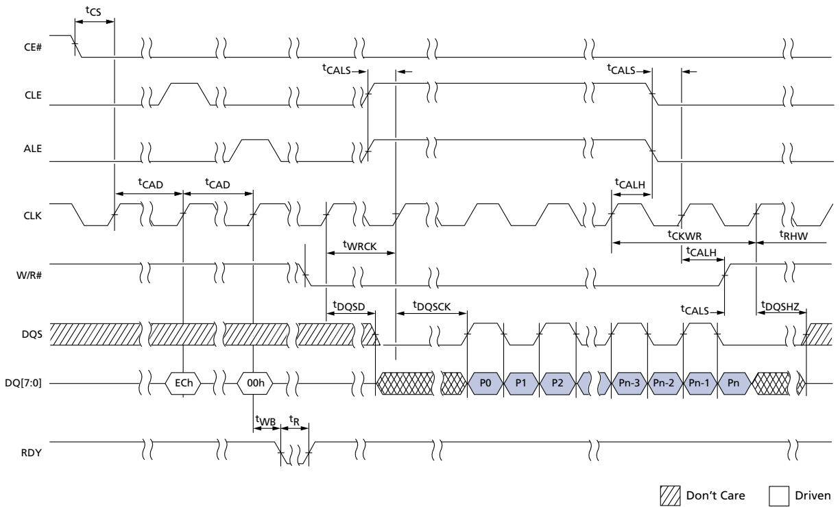
Figure 89: READ PARAMETER PAGE Operation
