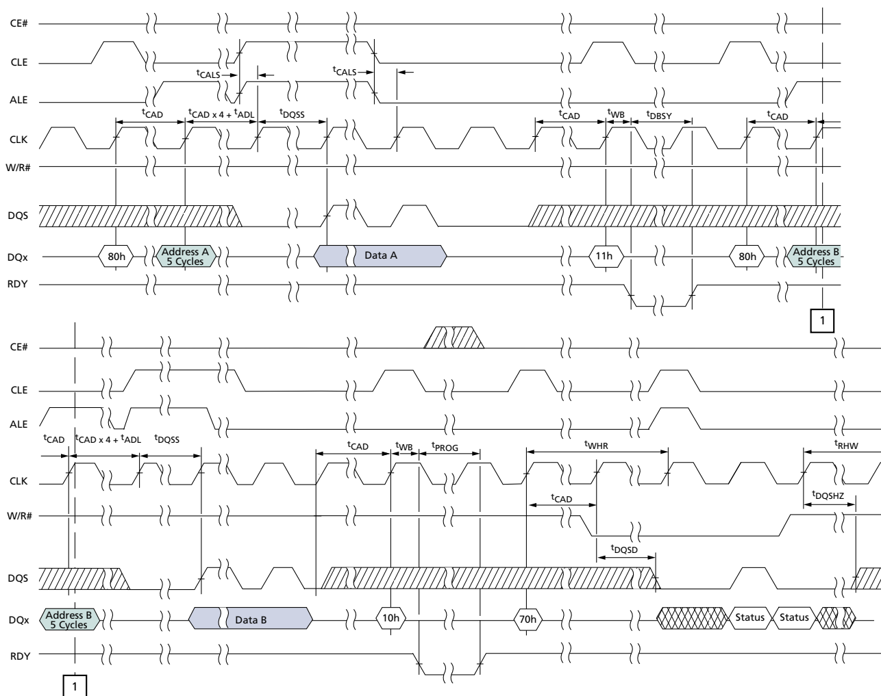
Figure 101: Multi-Plane Program Page
