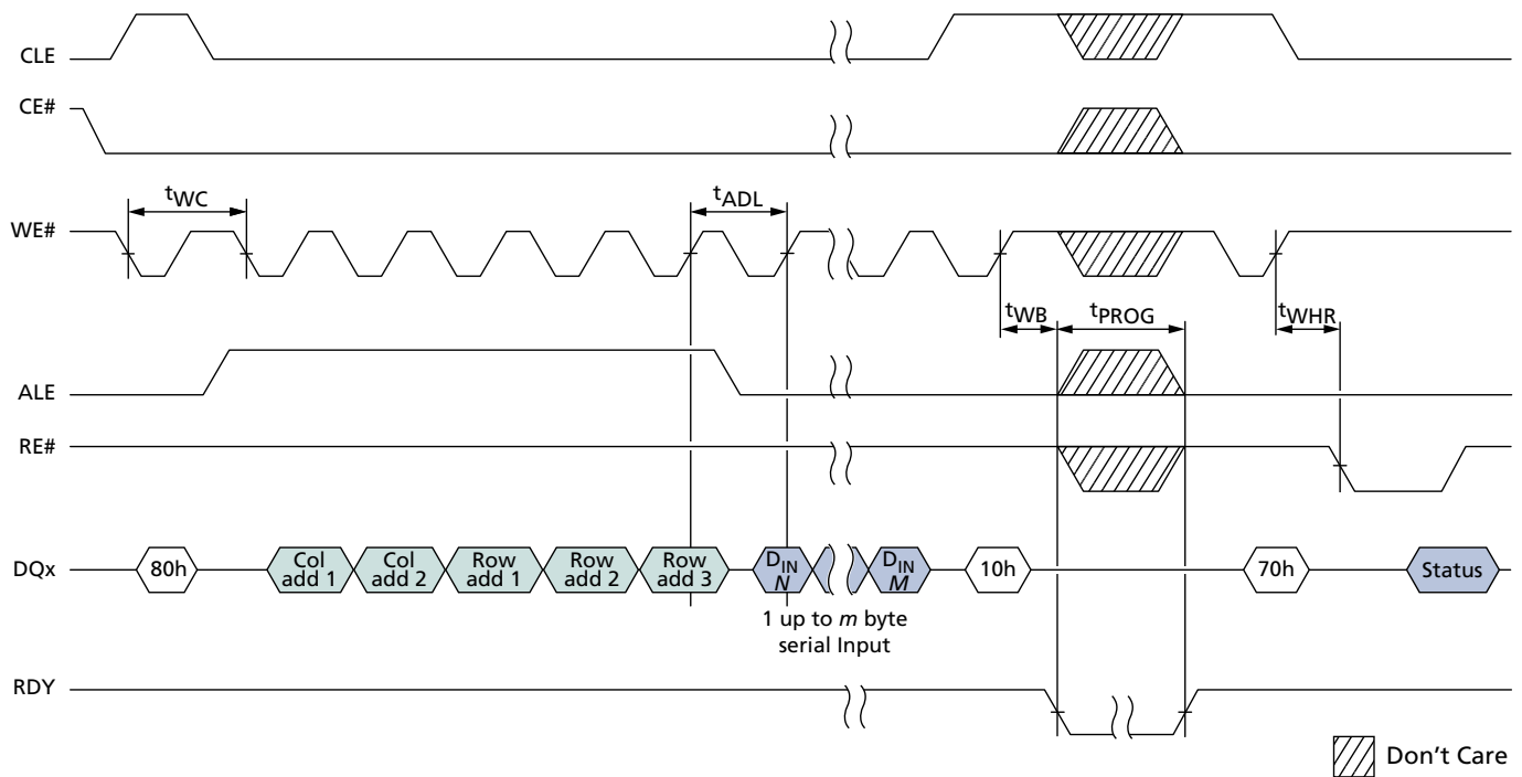
Figure 76: PROGRAM PAGE Operation
