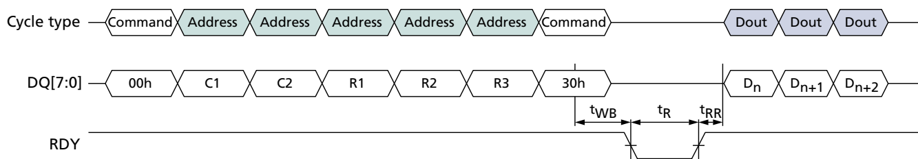
Figure 44: READ PAGE (00h-30h) Operation
