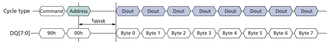
Figure 32: READ ID (90h) with 00h Address Operation
