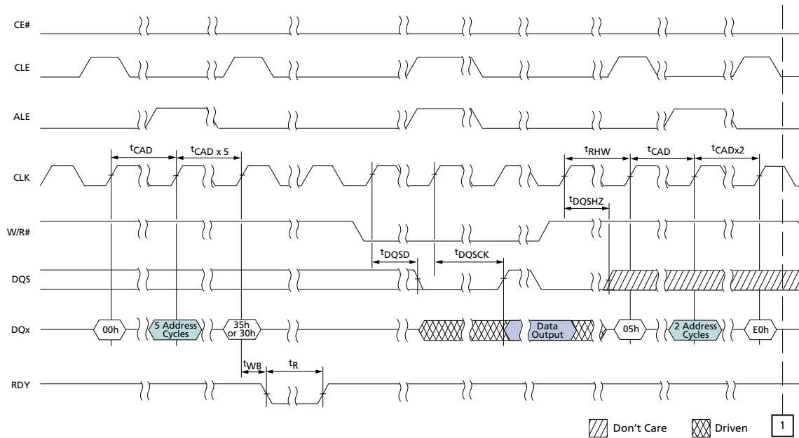
Figure 103: COPYBACK (1 of 3)
