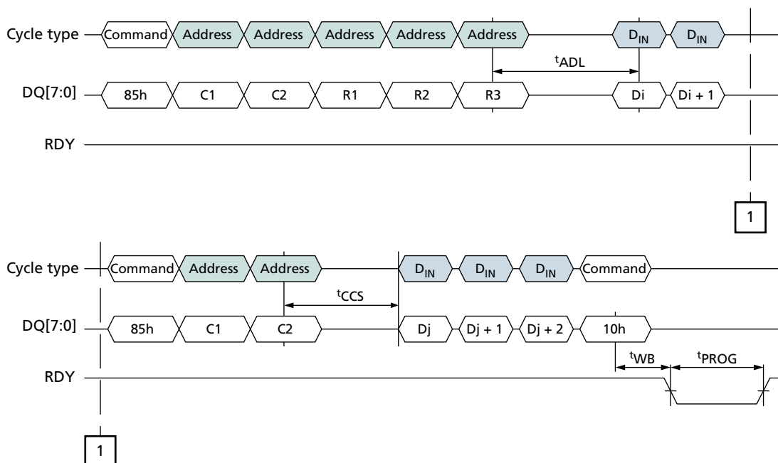
Figure 58: COPYBACK PROGRAM (85h-10h) with CHANGE WRITE COLUMN (85h) Operation
