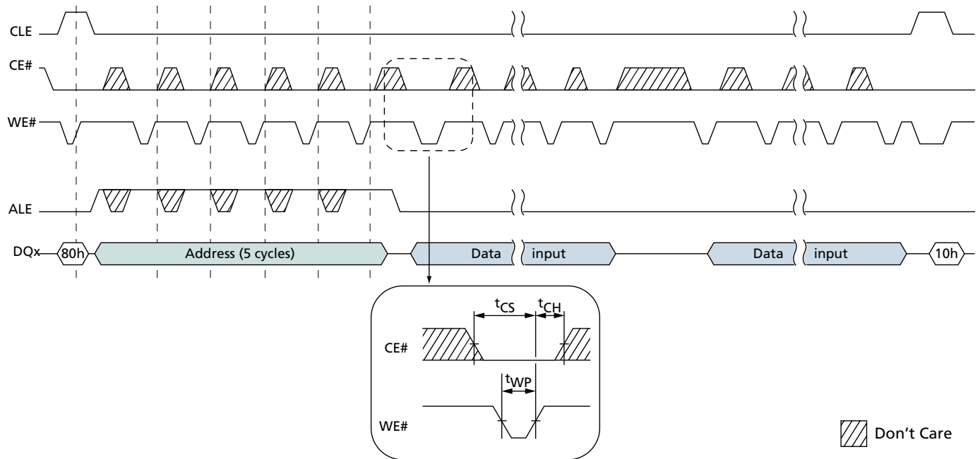
Figure 78: PROGRAM PAGE Operation with CHANGE WRITE COLUMN
