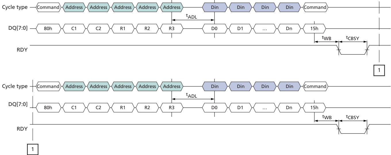
Figure 51: PROGRAM PAGE CACHE (80h–15h) Operation (End)
