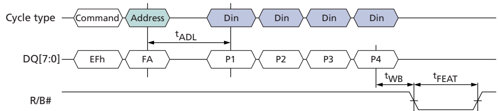
Figure 34: SET FEATURES (EFh) Operation
