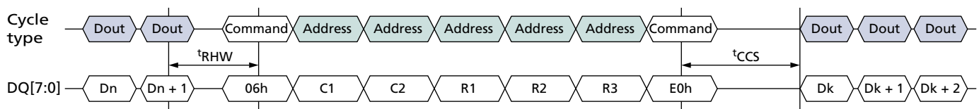
Figure 41: CHANGE READ COLUMN ENHANCED (06h-E0h) Operation
