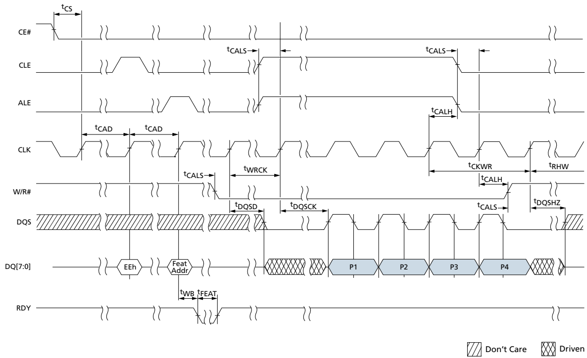
Figure 85: GET FEATURES Operation
