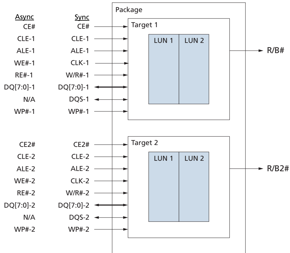
Figure 8: Device Organization for Four-Die Package with CE# and CE2# (BGA)
