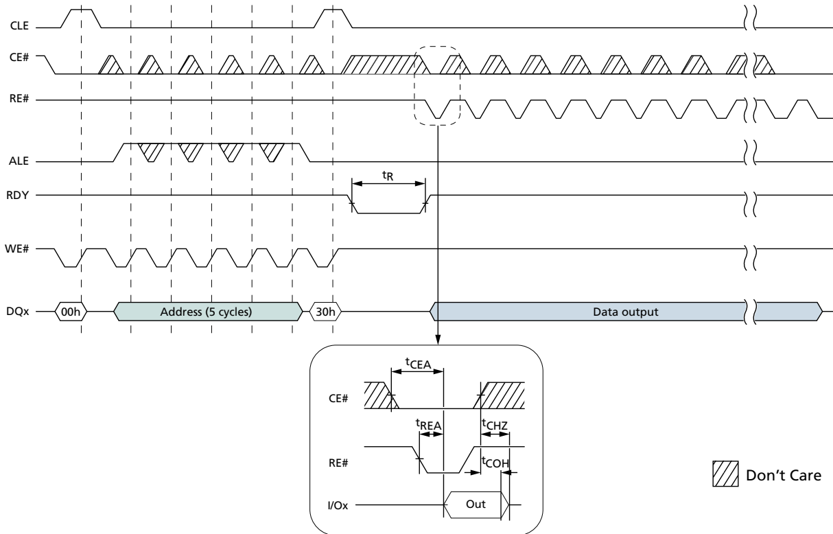
Figure 71: READ PAGE Operation with CE# "Don't Care"
