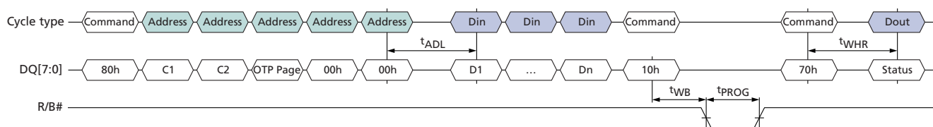
Figure 60: PROGRAM OTP PAGE (80h-10h) Operation
