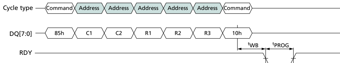
Figure 58: COPYBACK PROGRAM (85h-10h) with CHANGE WRITE COLUMN (85h) Operation
