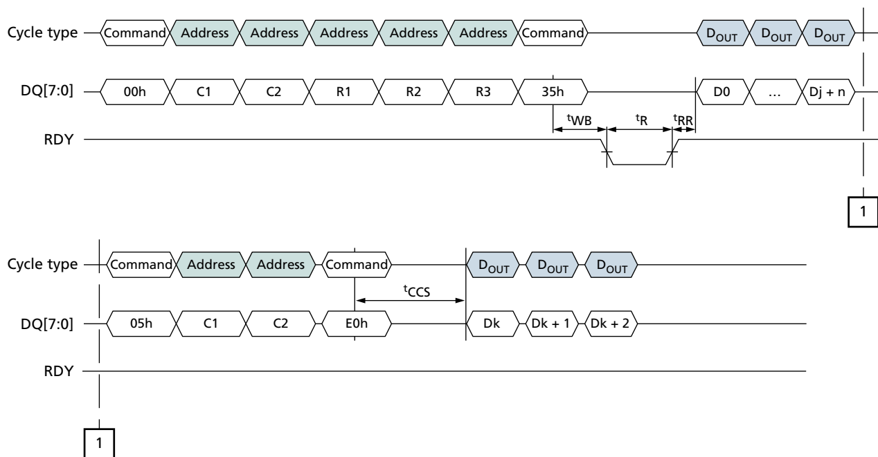
Figure 56: COPYBACK READ (00h-35h) with CHANGE READ COLUMN (05h-E0h) Operation
