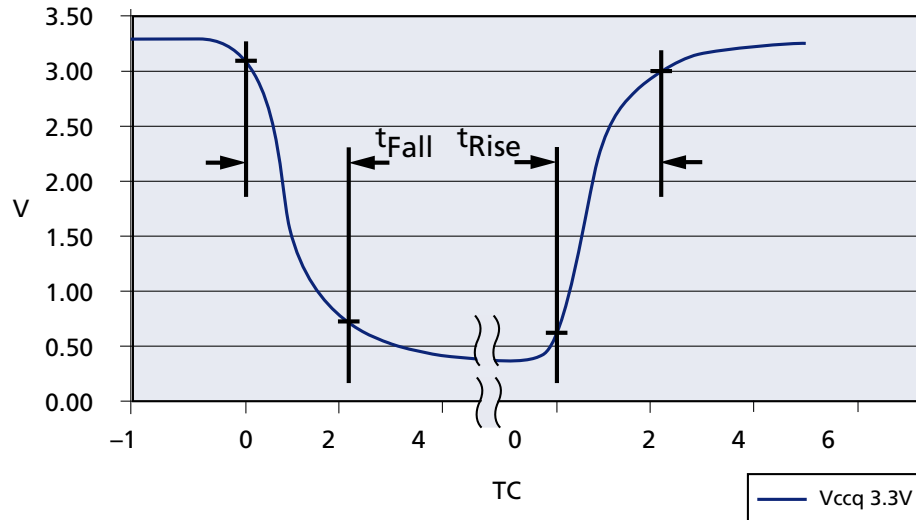
Figure 18: t_{\text{Fall}} and t_{\text{Rise}} ( V_{\text{CCQ}} = 2.7\text{-}3.6\text{V} )
