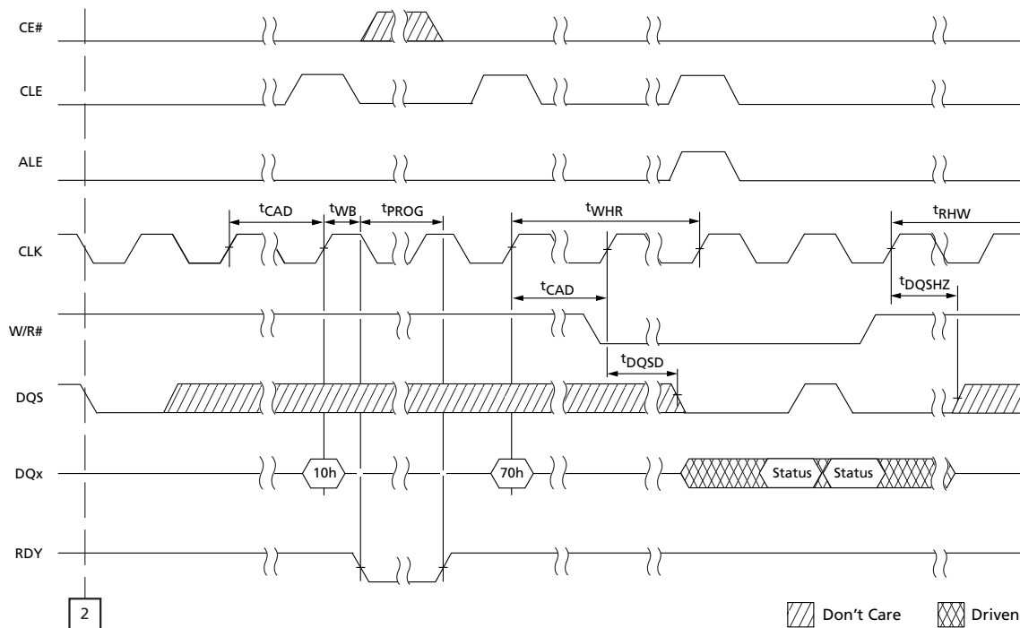
Figure 105: COPYBACK (3 of 3)
