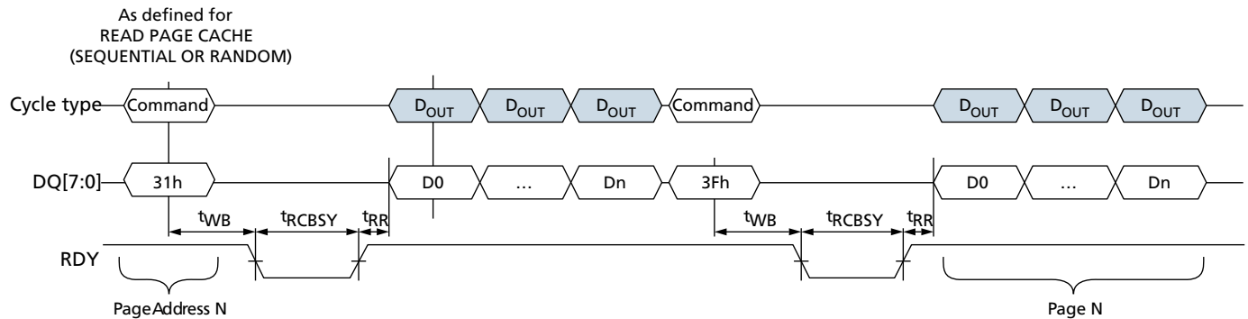
Figure 47: READ PAGE CACHE LAST (3Fh) Operation
