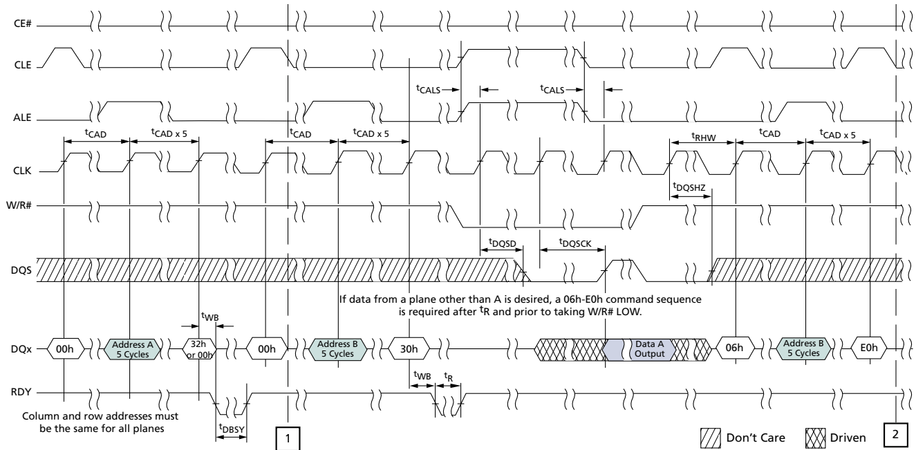
Figure 96: Multi-Plane Read Page (1 of 2)
