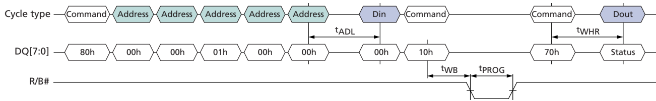
Figure 62: PROTECT OTP AREA (80h-10h) Operation
