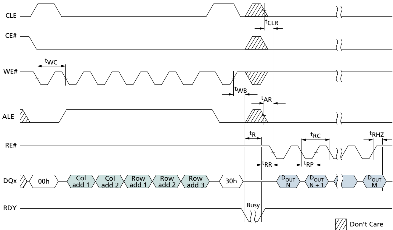
Figure 70: READ PAGE
