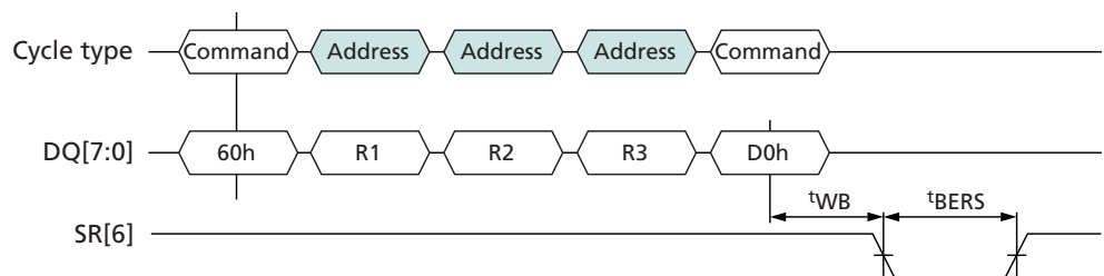
Figure 53: ERASE BLOCK (60h-D0h) Operation
